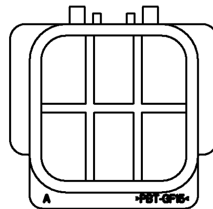
6 POS 2040594-4 SCALE 2:1
