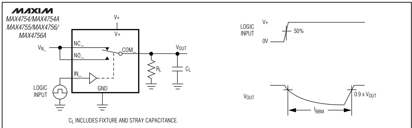
Figure 2. Break-Before-Make Interval
