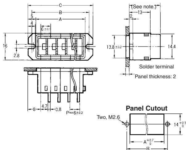
A7MA-1□□ Solder Terminals
