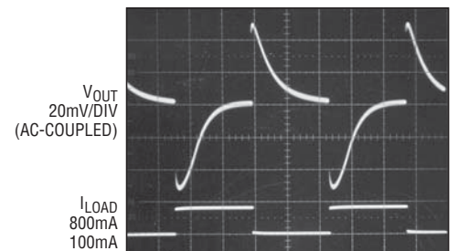
Output Voltage Transient Step Response Waveform (LDO Mode)
