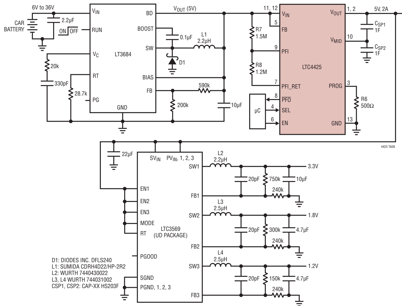
Embedded Automotive Backup Controller
