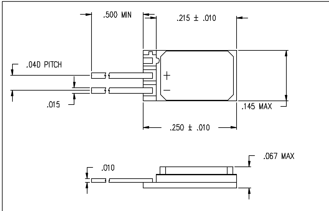
PACKAGE OPTION -01
