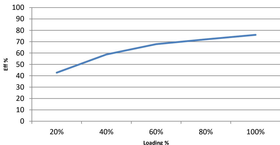
AM1P-4824SZ Efficiency vs. Loading
