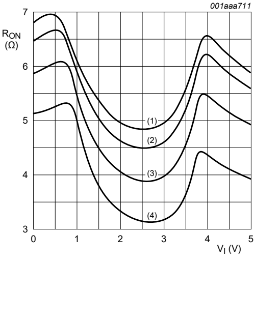
Fig. 11. ON resistance as a function of input voltage; V_{CC} = 5.0 V
