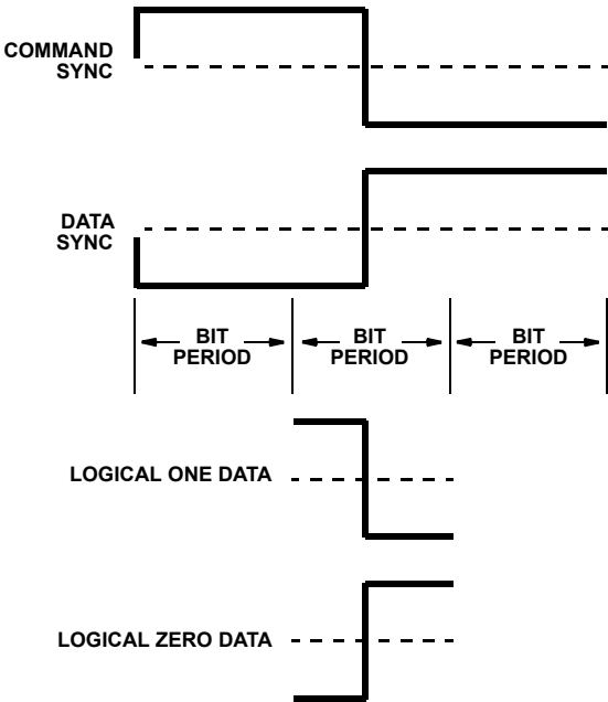
FIGURE 8. MIL-STD-1553 CHARACTER FORMATS
