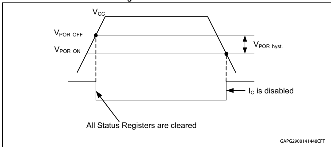
Figure 4. Power-on reset
