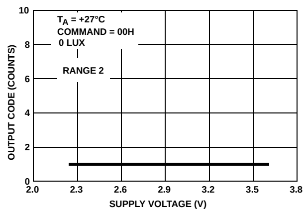
FIGURE 14. OUTPUT CODE FOR 0 LUX vs SUPPLY VOLTAGE
