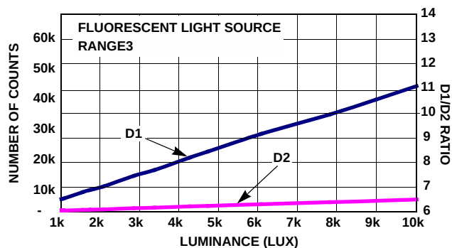
FIGURE 8. D1 AND D2 FLUORESCENT LIGHT SOURCE RESPONSE
