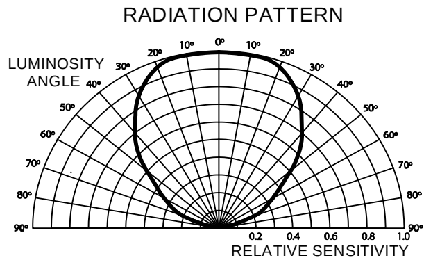
FIGURE 12. RADIATION PATTERN
