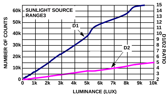
FIGURE 10. D1 AND D2 SUNLIGHT RESPONSE
