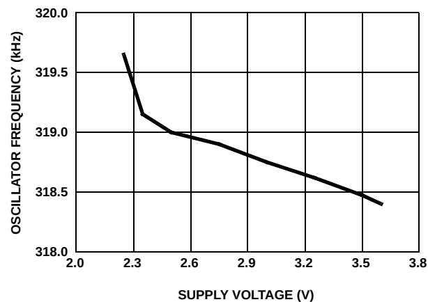
FIGURE 16. OSCILLATOR FREQUENCY vs SUPPLY VOLTAGE
