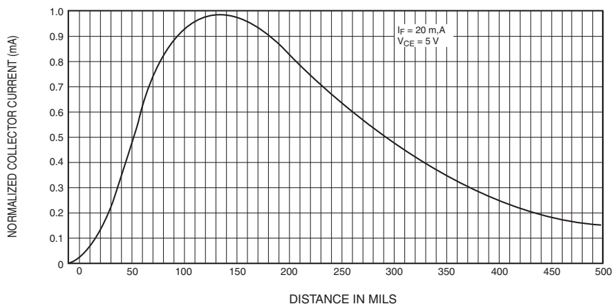
Fig. 5 Normalized Collector Current vs. Distance
