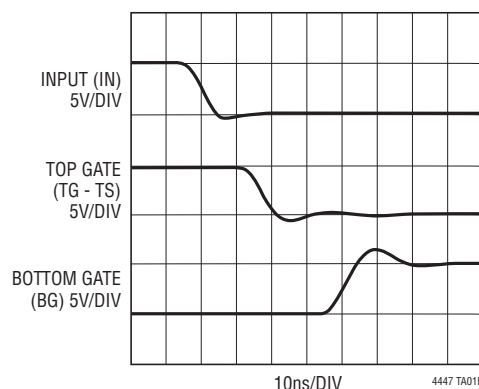
LTC4447 Driving 3000pF Capacitive Loads
