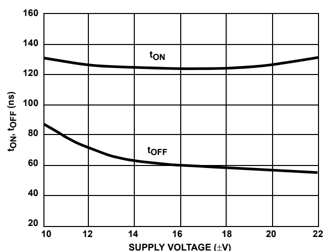
FIGURE 17. SWITCHING TIME vs POWER SUPPLY VOLTAGE (DG441)
