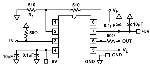
FIGURE 2C. SCHEMATIC
