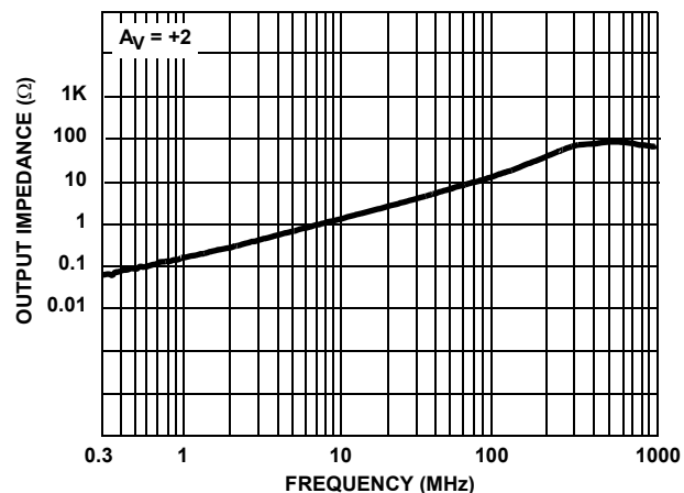
FIGURE 20. OUTPUT IMPEDANCE
