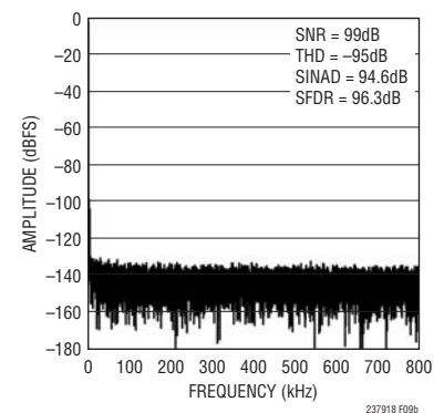
Figure 9b. 32k Point FFT Plot with f_{IN} = 2kHz for Circuit Shown in Figure 9a
