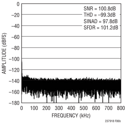
Figure 6b. 32k Point FFT Plot with f_{IN} = 2\text{kHz} for Circuit Shown in Figure 6a
