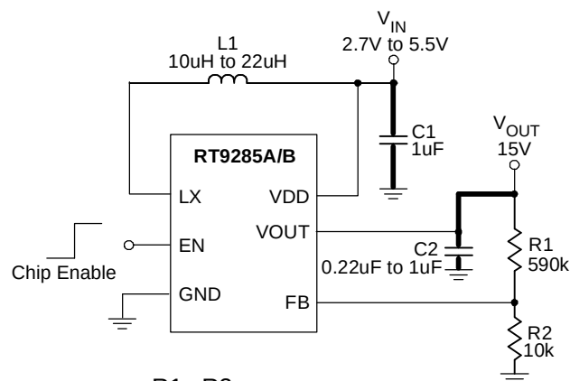
Figure 5. Application for Constant Output Voltage
