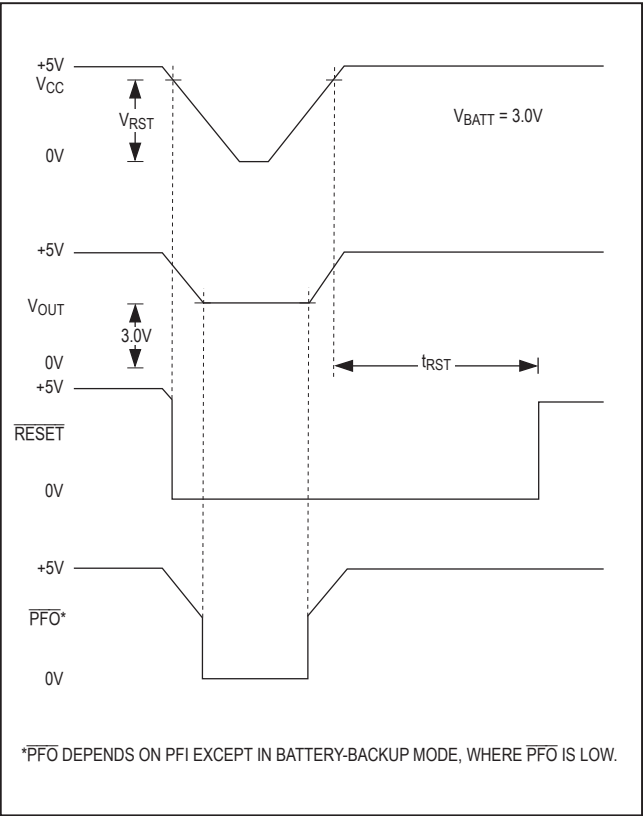
Figure 2. Timing Diagram
