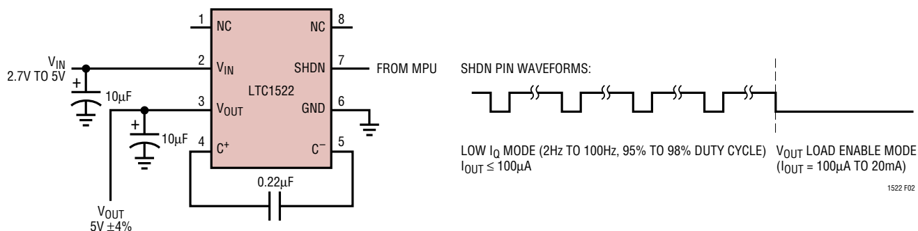
Figure 2. Ultralow Quiescent Current (&lt;2.1µA) Regulated Supply
