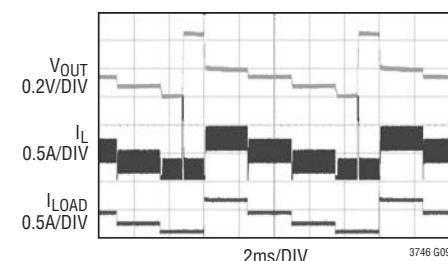
Adaptive LED Bus Voltage IV
