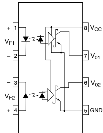
Figure 2. Dual-channel Circuit Drawing (HCPL0637, HCPL0638 and HCPL0639)
