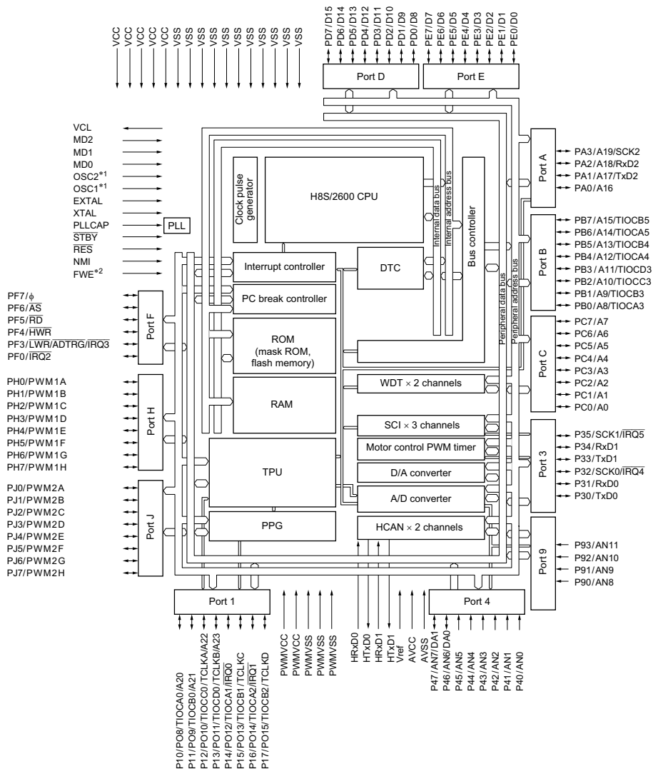
Figure 1-1 (a) shows an internal block diagram of the H8S/2636.
