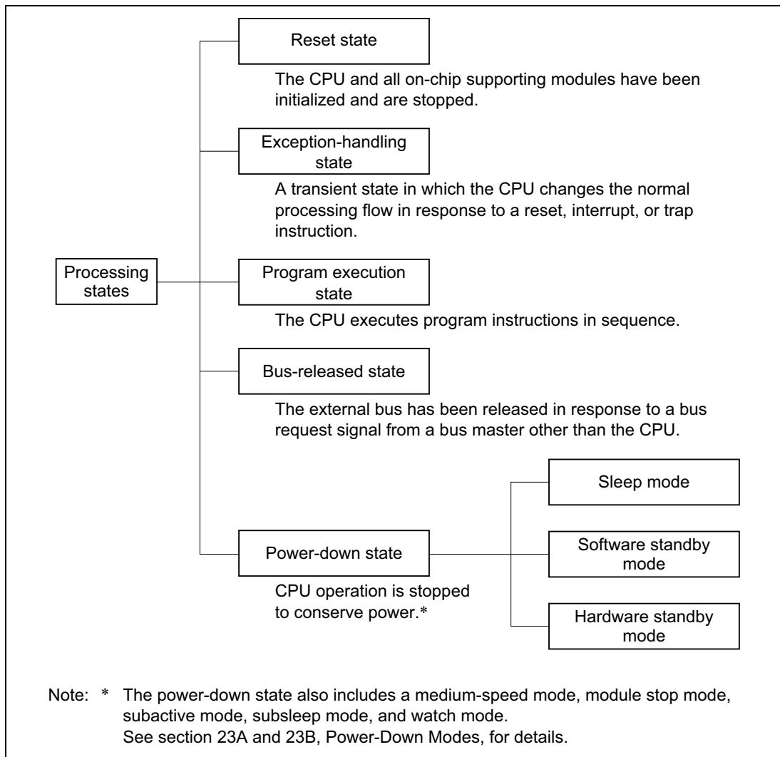
Figure 2-14 Processing States
