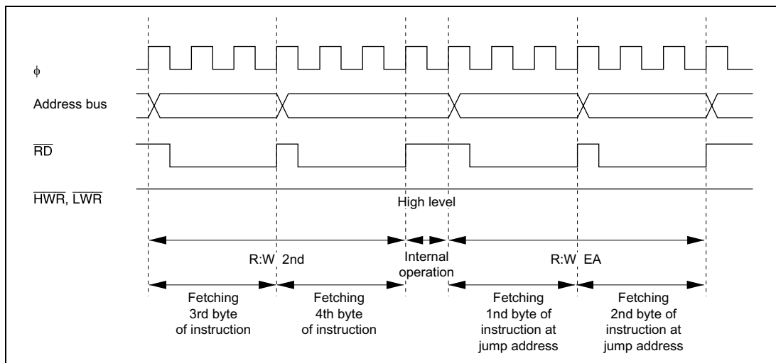
Figure A-1 Address Bus, \overline{\text{RD}} , \overline{\text{HWR}} , and \overline{\text{LWR}} Timing (8-Bit Bus, Three-State Access, No Wait States)
