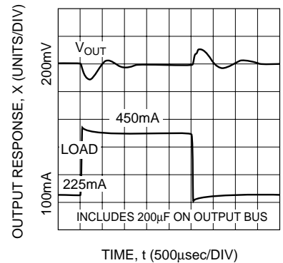
LOAD TRANSIENT RESPONSE 200µF
