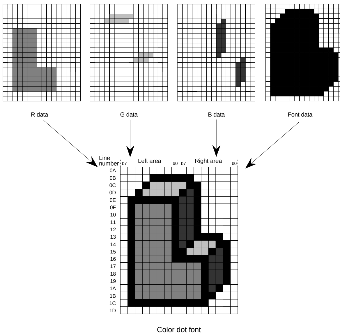
Fig. 8.10.16 Color dot Font Data Storing Address
