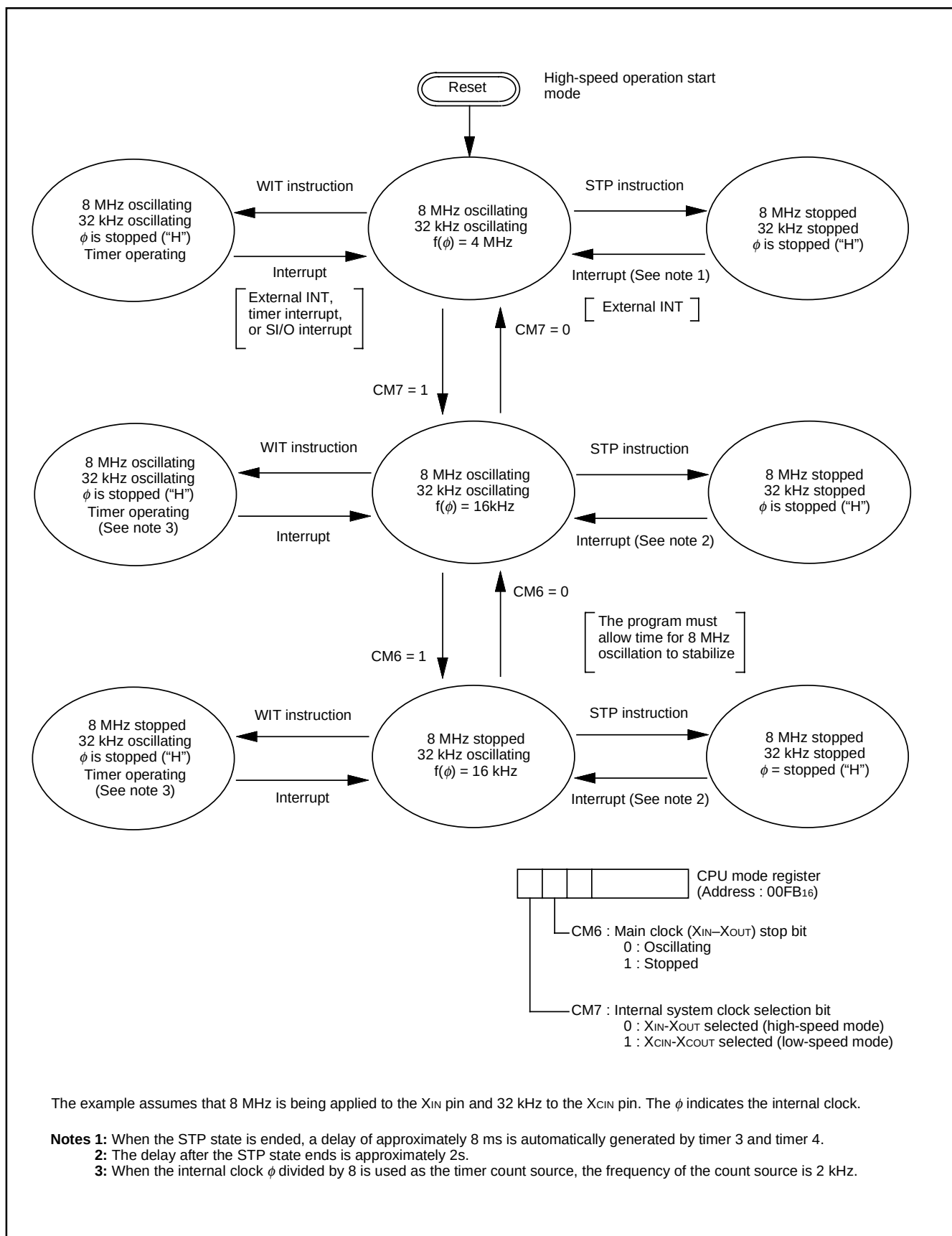
Fig.8.13.6 State Transitions of System Clock
