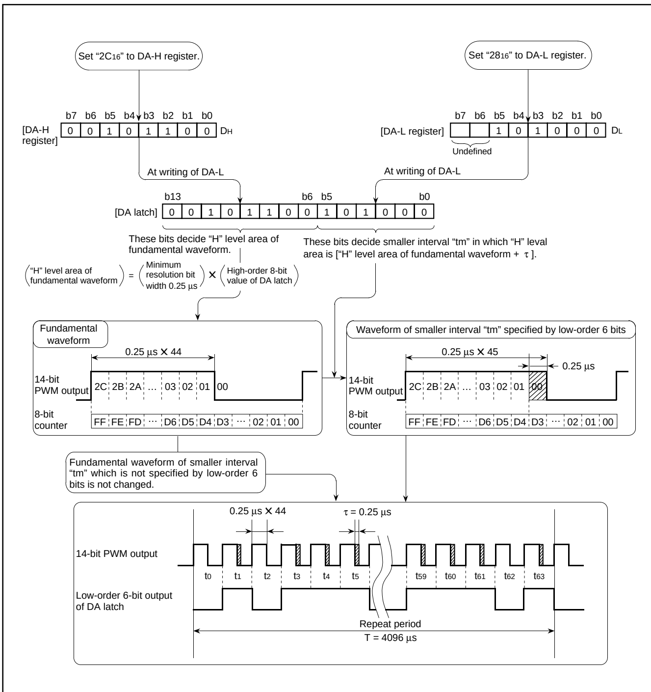
Fig. 8.7.3 14-bit PWM Output Example ( f(X_{IN}) = 8\text{MHz} )
