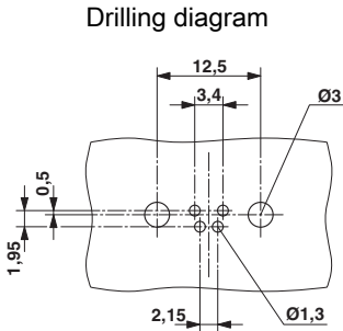
Drilling diagram
