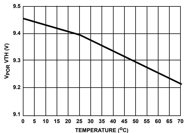
FIGURE 4. V_{CC} POWER ON RESET VTH vs TEMPERATURE
