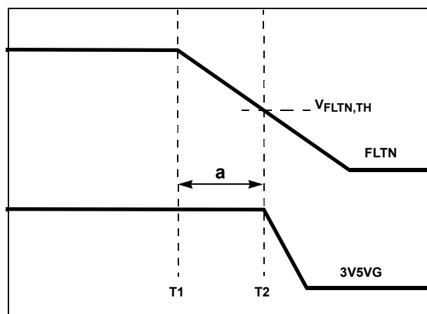
FIGURE 5. TIMING DIAGRAM
