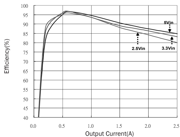
Figure 10. Efficiency(V IN )
