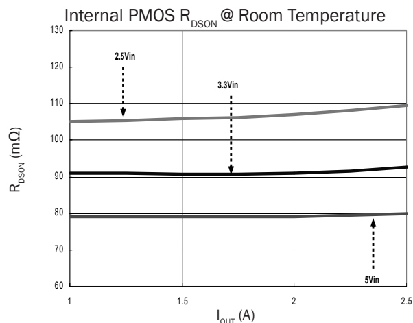
Figure 11. High-Side P-MOSFET
