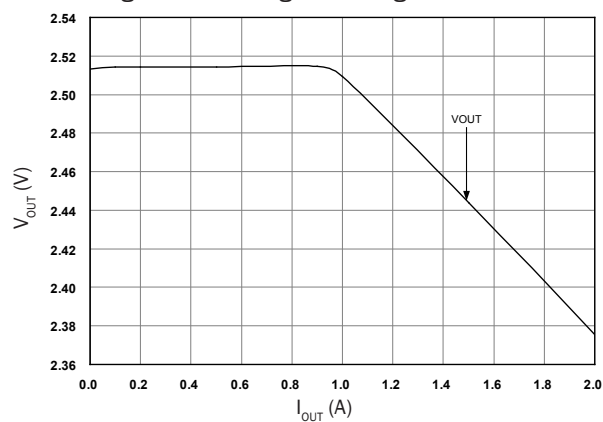
Figure 13. Loading Regulation
