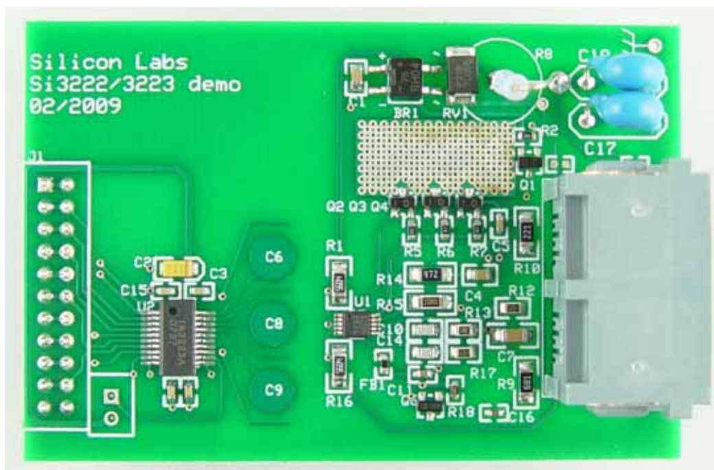
Figure 1. IA3222/3223 Demo Board
