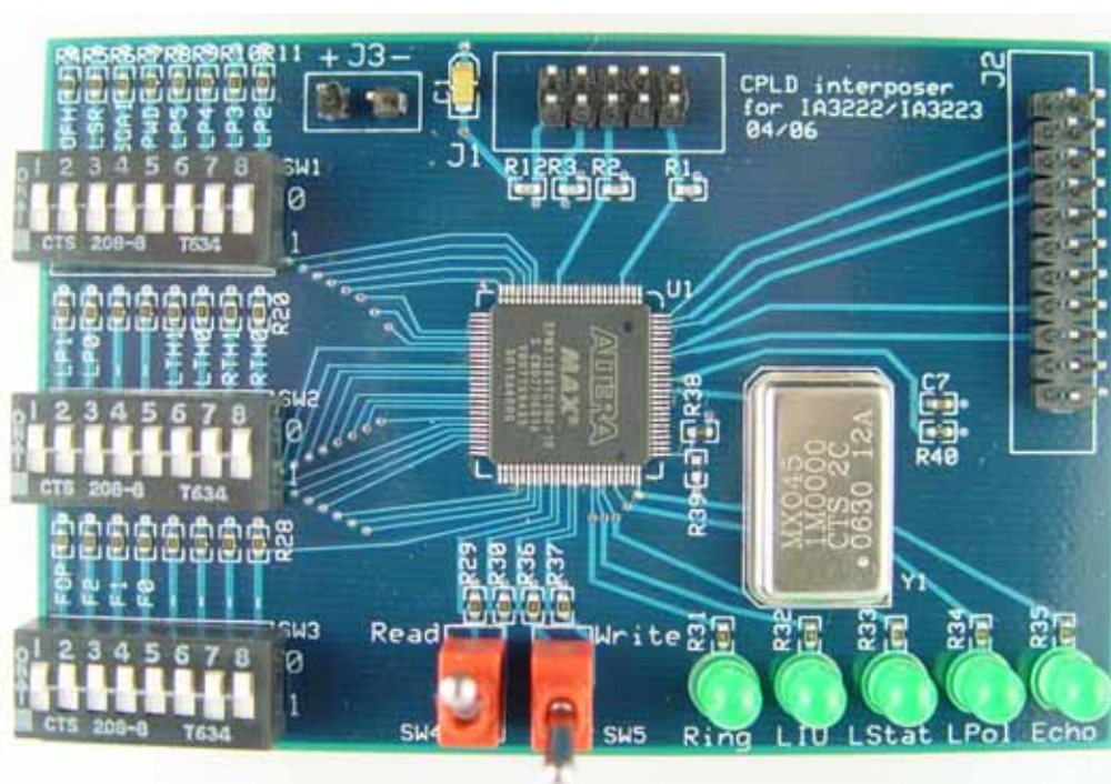
Figure 2. CPLD Interposer
