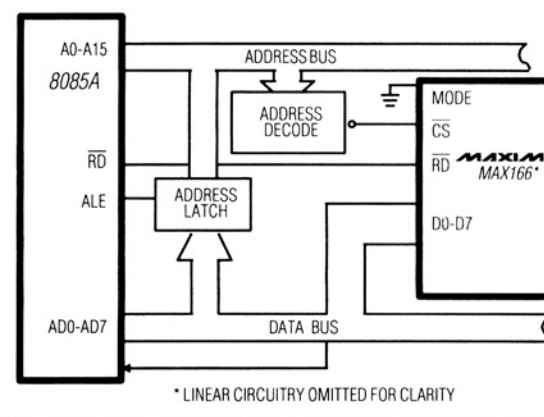
Figure 10. MAX166 to 8085A Asynchronous-Conversion Mode Interface
