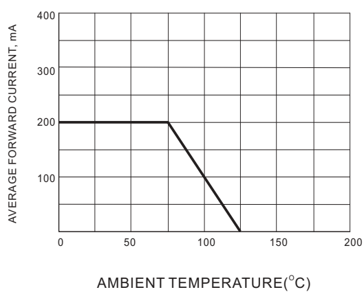
FIG. 4 FORWARD CURRENT DERATING
