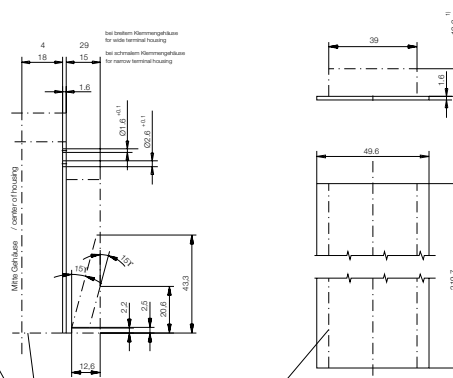
Querplatine / Crosswise circuit board
