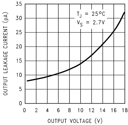
Output Leakage Current vs. Output Voltage LMC7225
