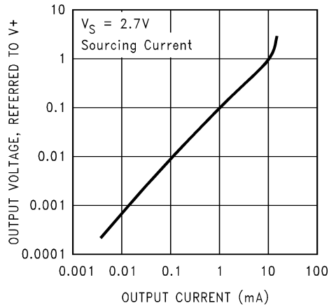
Output Voltage vs. Output Current LMC7215
