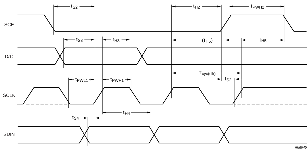
Fig.15 Serial interface timing.
