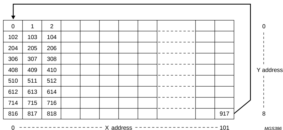
Fig.6 Sequence of writing data bytes into RAM with horizontal addressing ( V = 0 ).
