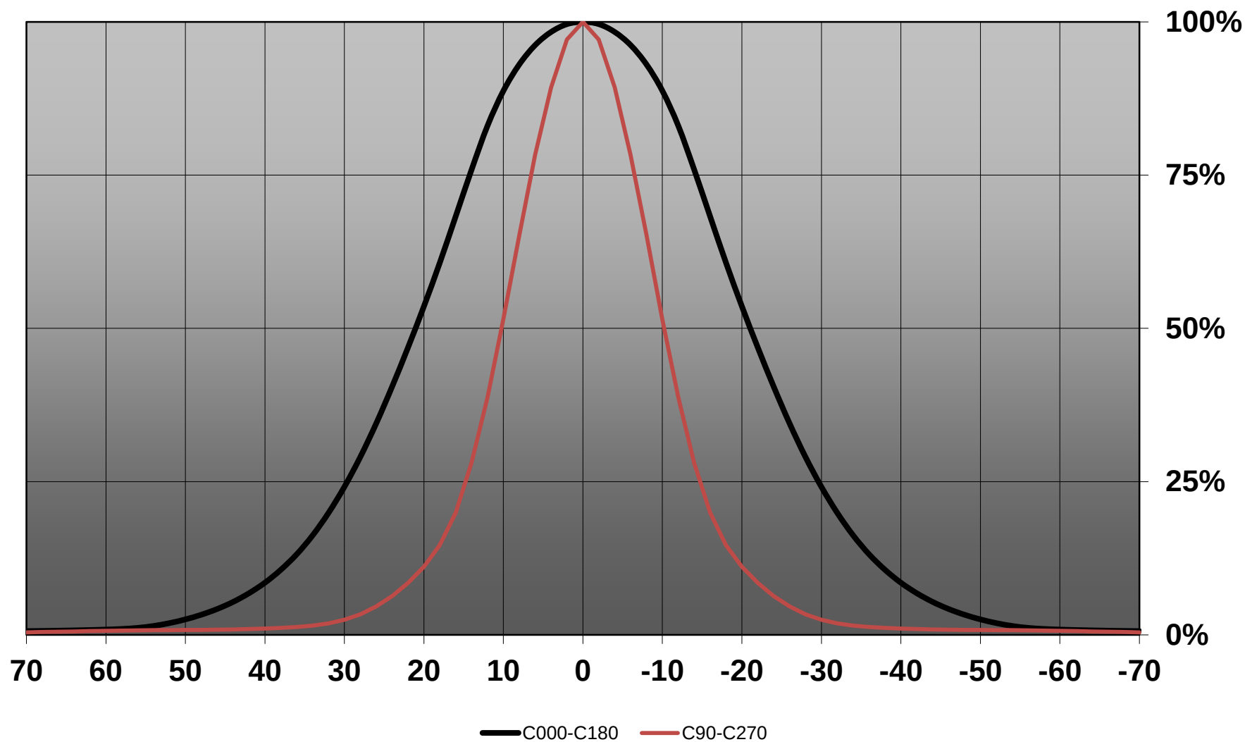
Relative intensity of FA11912_CXM-O_(XM-L2)
