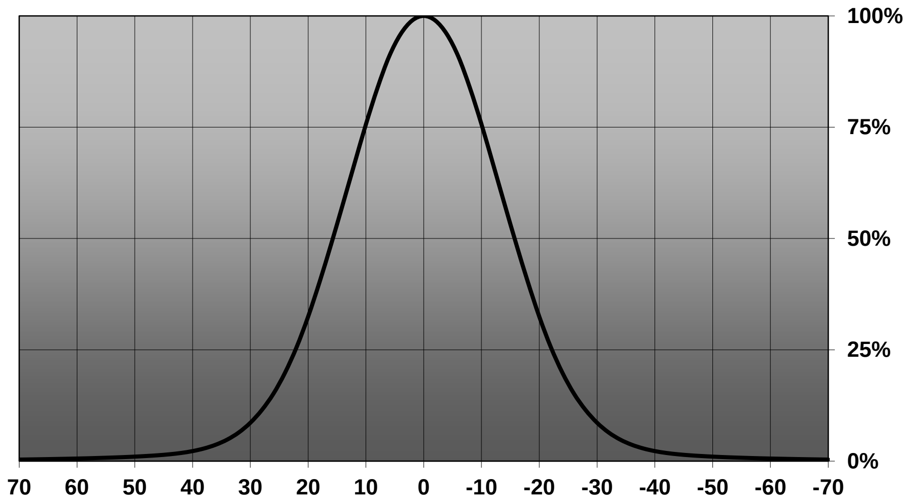
Relative intensity of FA11911_CXM-M_(XM-L2)
