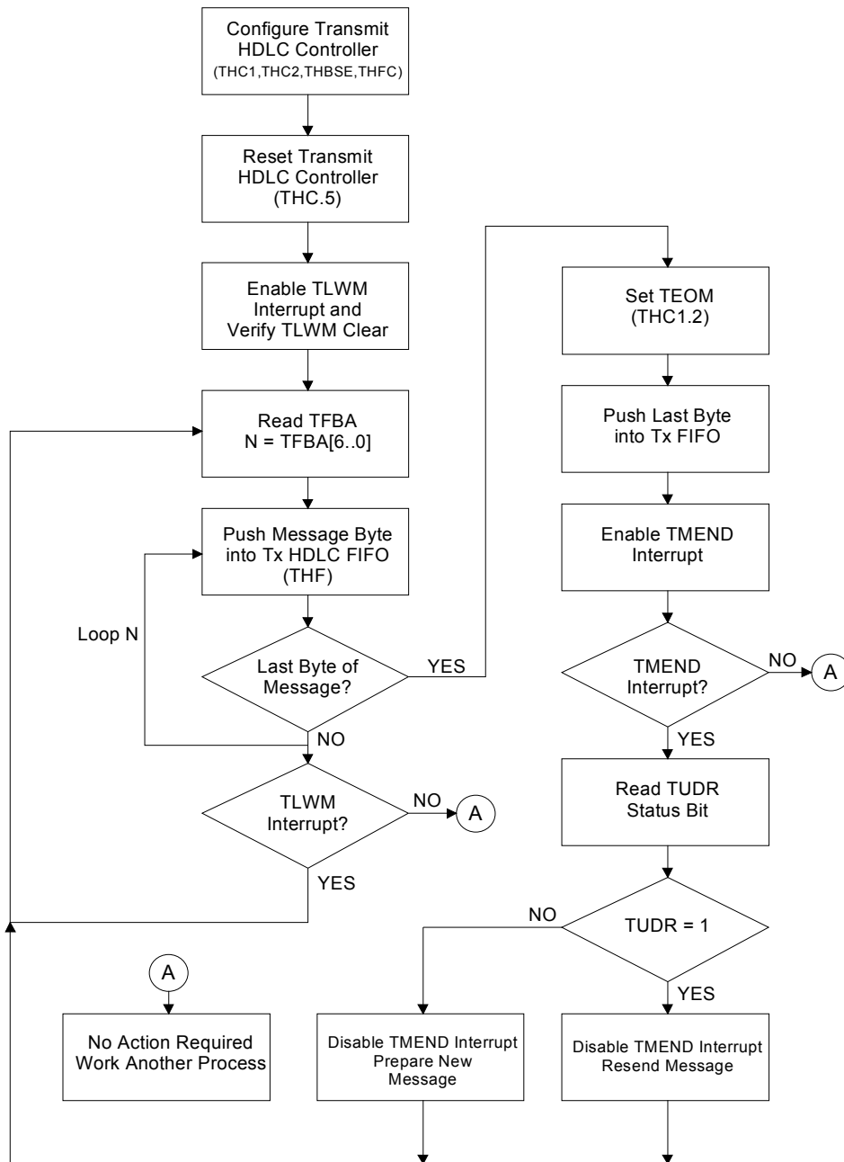
Figure 8-10. HDLC Message Transmit Example
