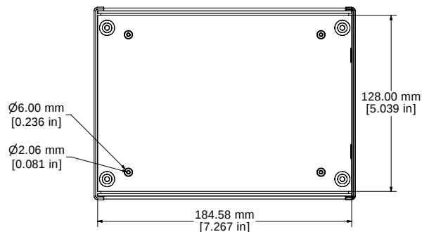
BASE - INSIDE
