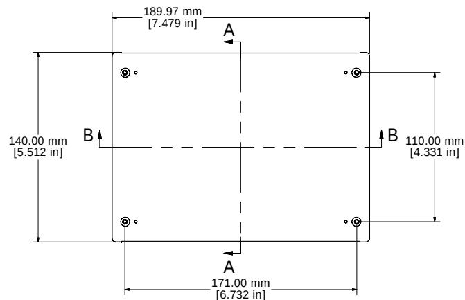
ASSEMBLY - BOTTOM
