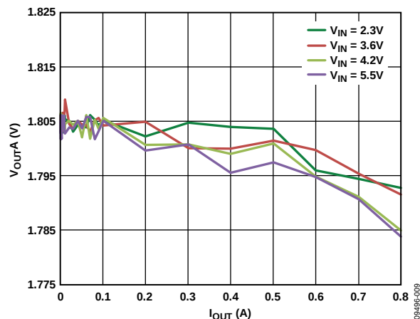
Figure 9. Load Regulation Across Input Voltage, V_{OUT} = 1.8\text{ V} , PWM Mode
