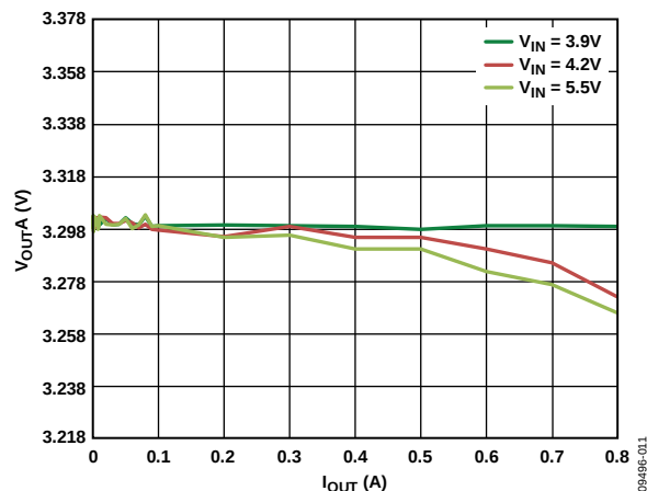
Figure 11. Load Regulation Across Input Voltage, V_{OUT} = 3.3\text{ V} , PWM Mode
