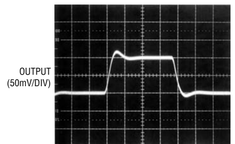
Small-Signal Transient Response ( I_S = 300\mu\text{A} per Amplifier)
