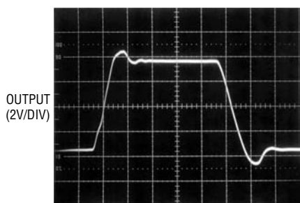
Large-Signal Transient Response ( I_S = 6\text{mA} per Amplifier)
