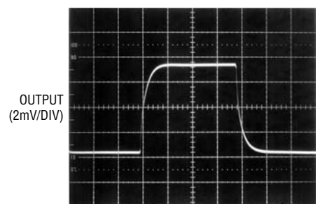
Large-Signal Transient Response ( I_S = 300\mu\text{A} per Amplifier)
