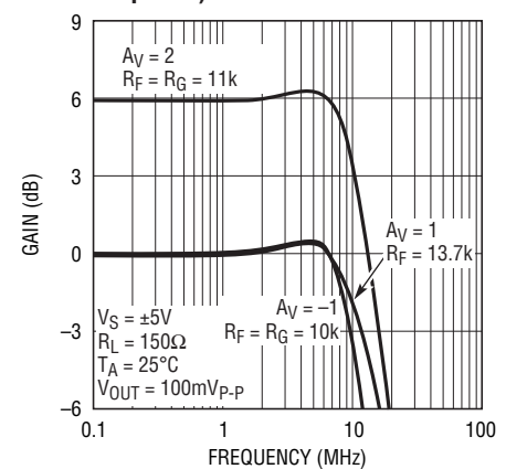
Frequency Response vs Closed Loop Gain ( I_S = 300μA per Amplifier)
