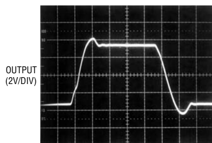
Large-Signal Transient Response ( I_S = 3\text{mA} per Amplifier)
