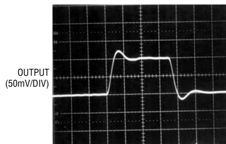
Small-Signal Transient Response ( I_S = 3\text{mA} per Amplifier)
