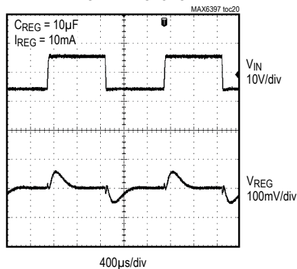
TRANSIENT RESPONSE
