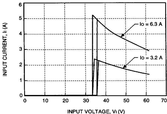
Figure 1. Typical FE150H Input Characteristics at Room Temperature
