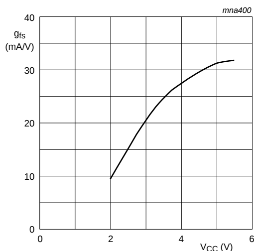
Fig 12. Typical forward transconductance g_{fs} as a function of the supply voltage at T_{amb} = 25^\circ\text{C}
