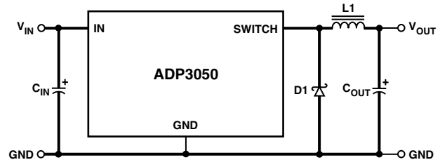
Figure 3. Main Switching Path
