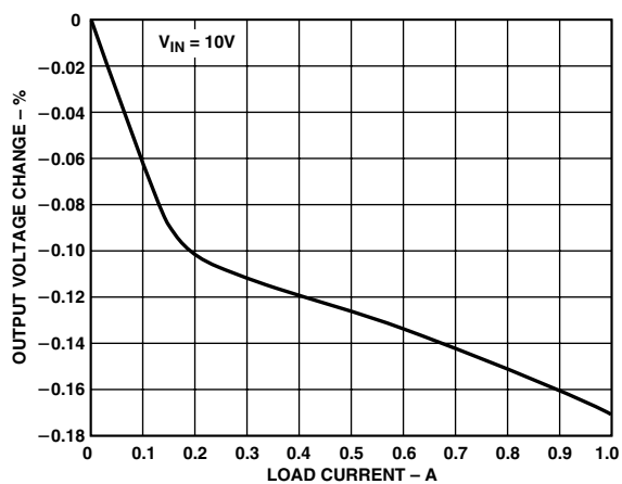
TPC 12. Load Regulation
