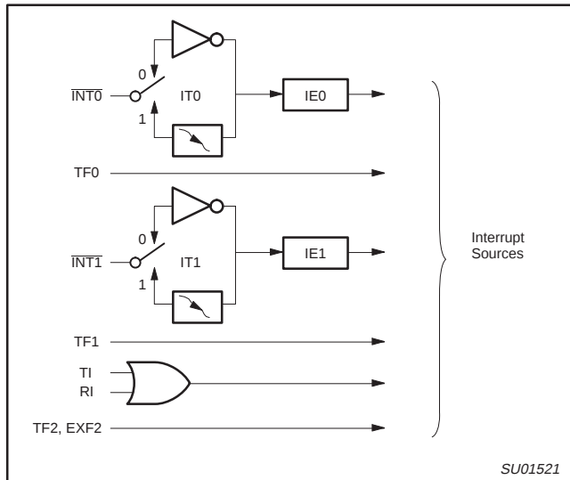
Figure 23. Interrupt Sources
