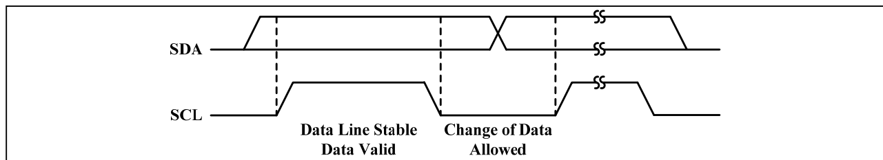
Figure 3 Bit transfer
