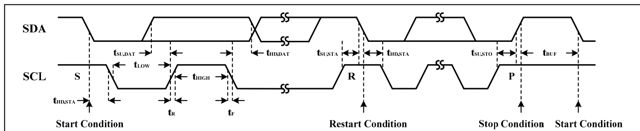
Figure 2 Interface timing
