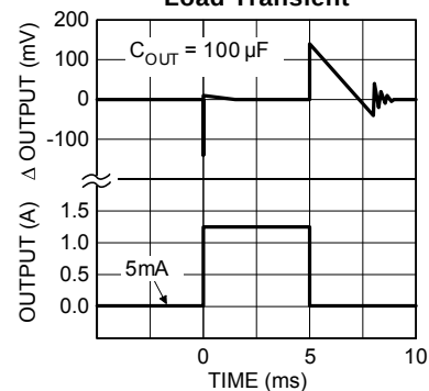
Load Transient
