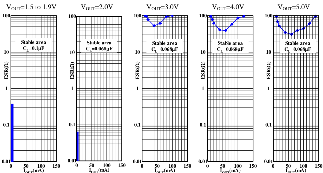
Figure 3. Stable operation area vs. voltage, current, and ESR
