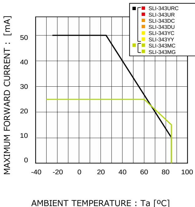
Fig.4 Derating
