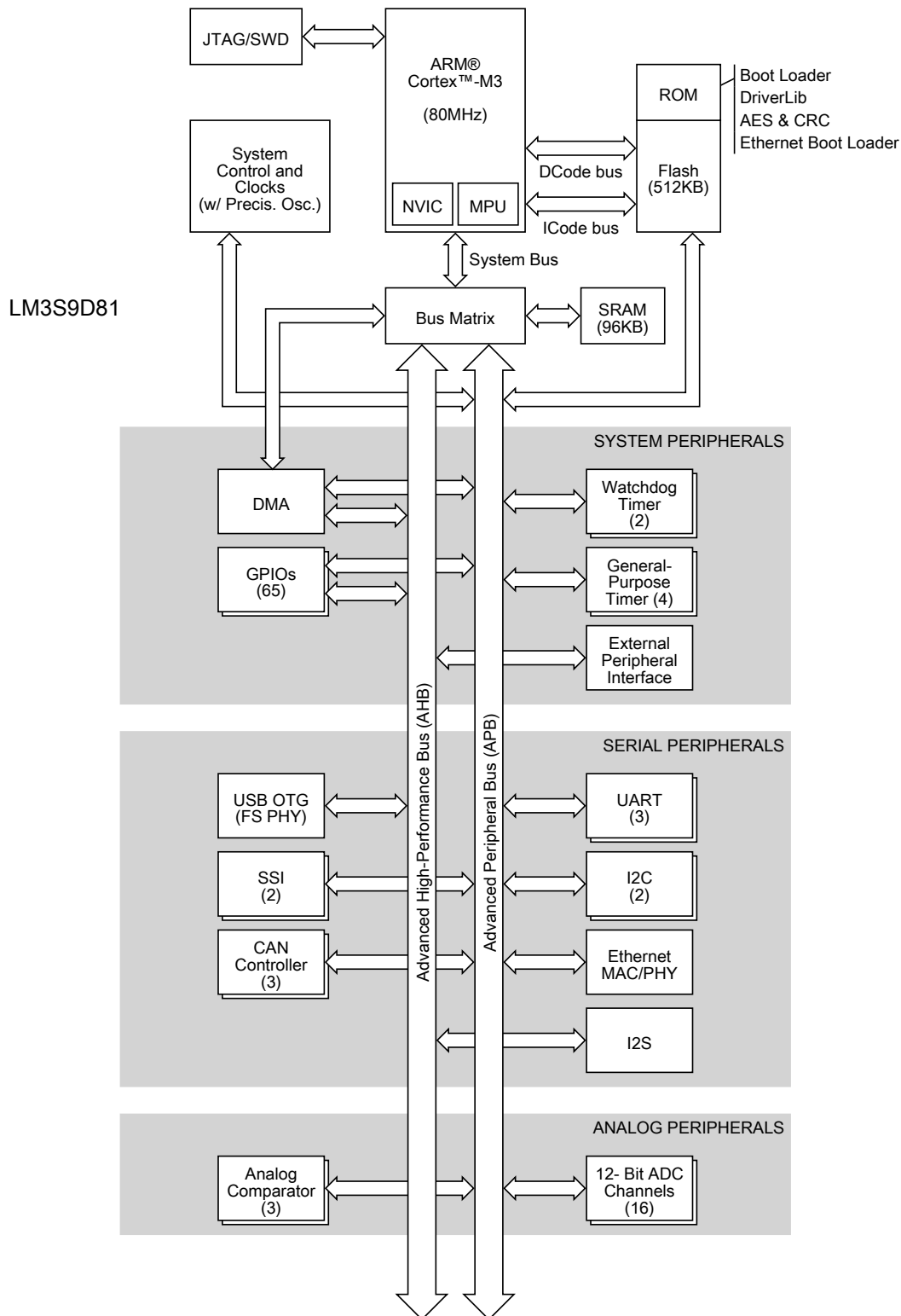
Figure 1-1. Stellaris LM3S9D81 Microcontroller High-Level Block Diagram
