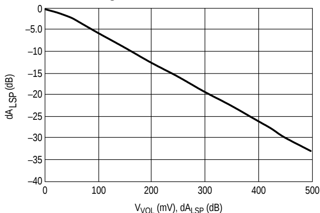
Figure 13. Volume Reduction
