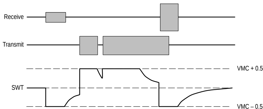
Figure 16. Switch-Over Behavior
