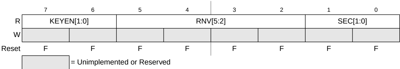
Figure 17-6. Flash Security Register (FSEC)
