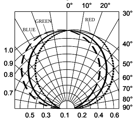
Radiation Diagram
